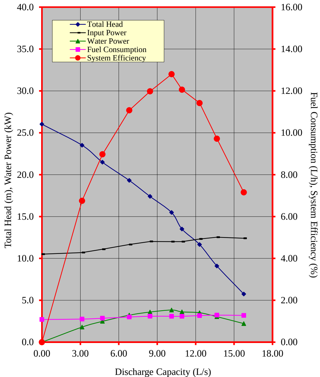
Figure 3. Performance characteristic curves of the YAMAHA YP30G self-priming centrifugal pumpset
