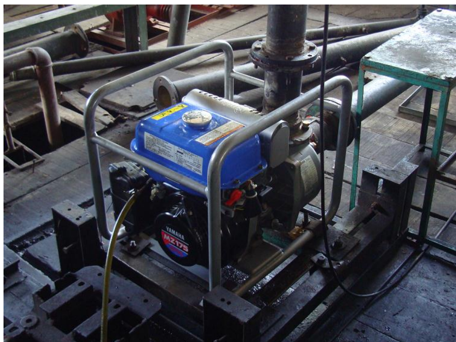
Figure 1. YAMAHA YP30G Pumpset on the test set-up
